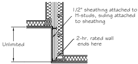
2-HR. Firewall wall offset with siding attachment
