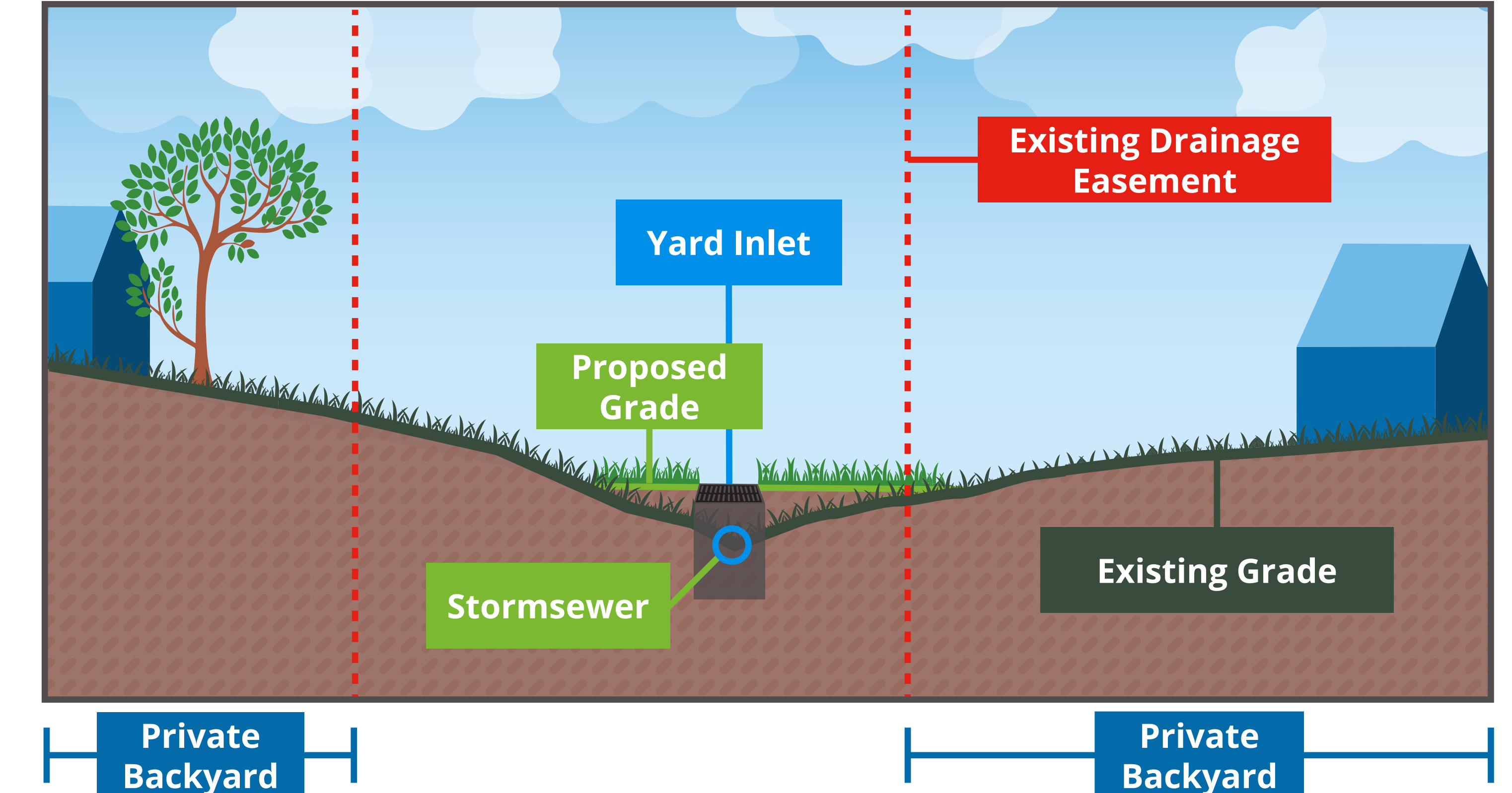
Typical Stormsewer Cross Section
