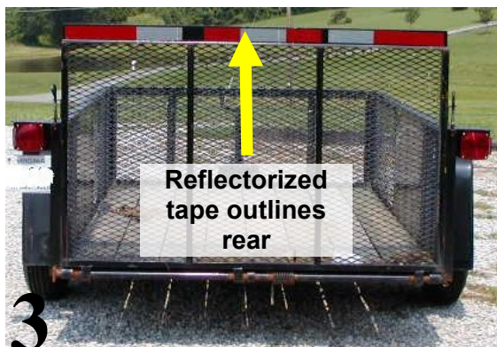
PHOTO 3: NO VIOLATION - This trailer has 100+ inches of reflectorized tape.
