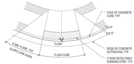
Sidewalk Access Ramp
