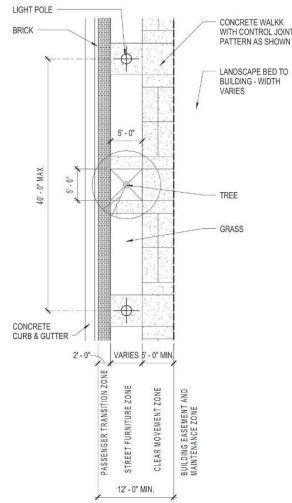
Low Traffic Interior Street
