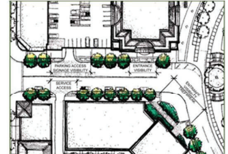
The line of street trees may need to be broken where parking access, critical signage, major hotel and theatre entrances, and arcades need to be seen from the street.
