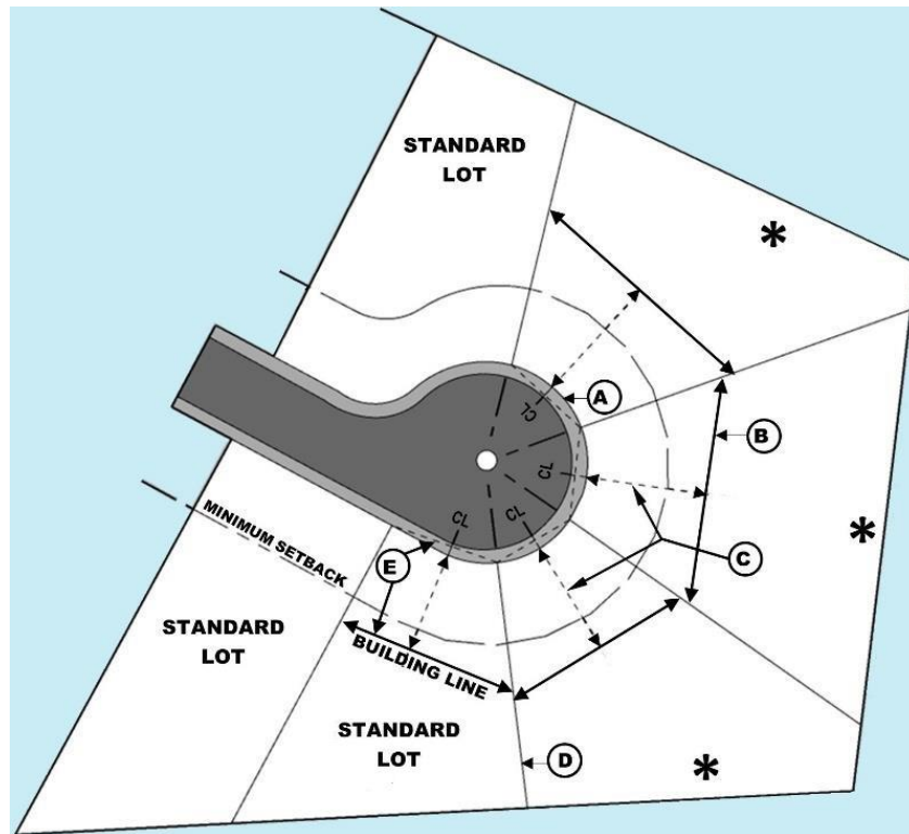
Figure 8302B: Lot width on cul-de-sac lots
