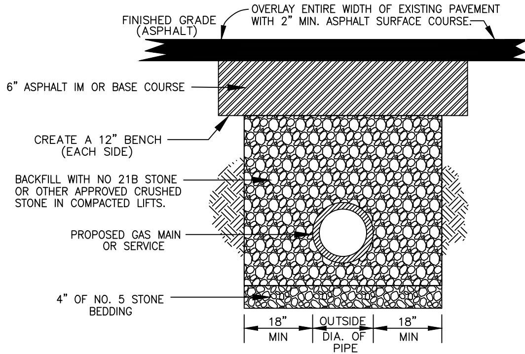
SKETCH SHOWING PAVEMENT OVERLAY FOR LONGITUDINAL OR MULTIPLE CUTS
